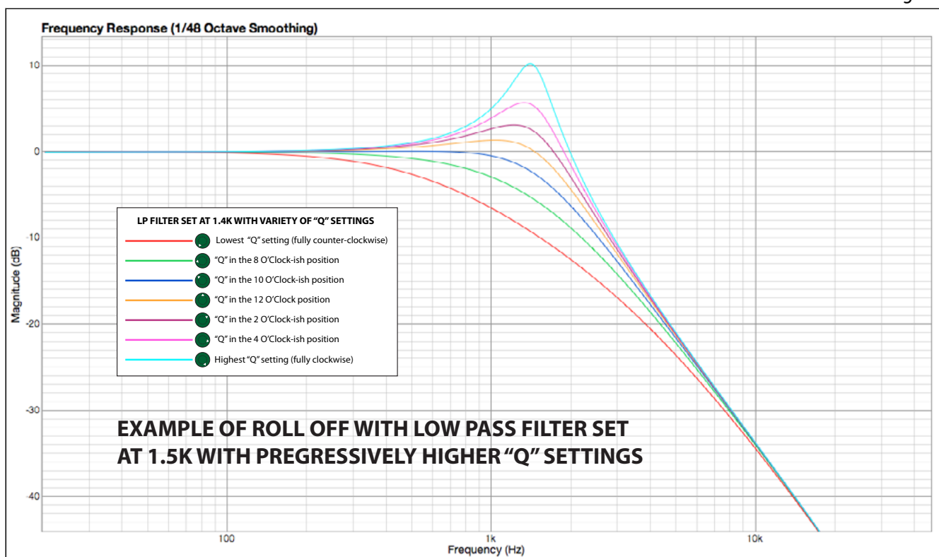
Fig. 6 allows you to better see how the slope and peaking develop as the “Q” control goes from the fully counter-clockwise position to the fully clockwise position.
